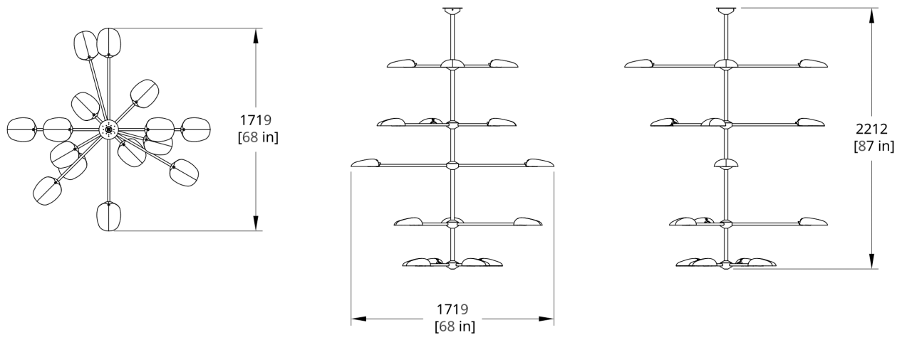
PT-16A5 Pilot Chandelier Five Tier Dimension
